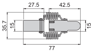
CKC-1007-11 CKC-7-11
