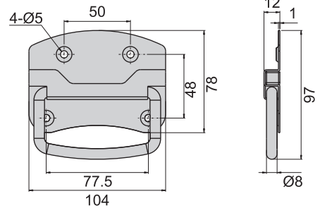
CKA-1006-4 CKA-6-4
