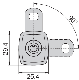
CPA-406-19-22
