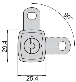
CPA-406-19-11
